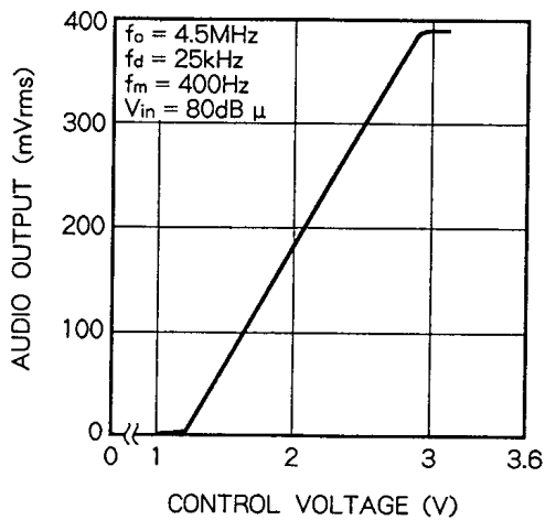
SOUND OUTPUT ELECTRONIC VOLUME CONTROL CHARACTERISTICS
