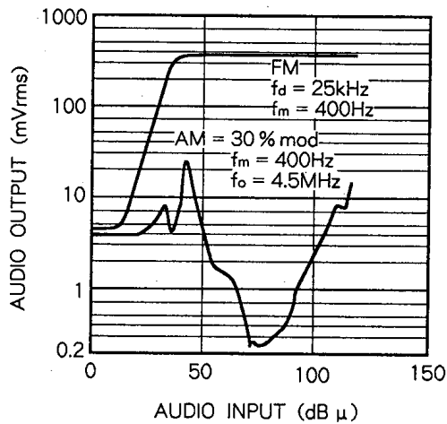
SIF LIMITING CHARACTERISTICS AND AMR CHARACTERISTICS
