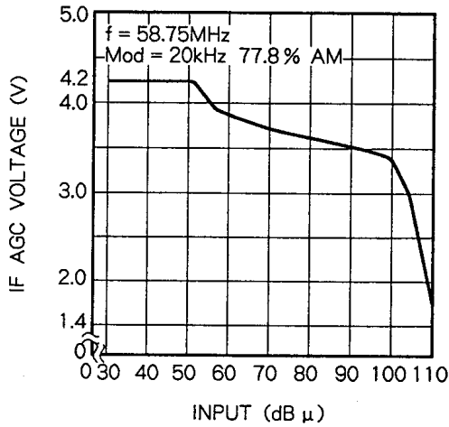
IF AGC CHARACTERISTICS (M51348AFP)
